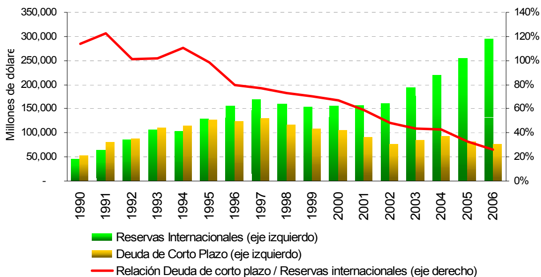
Chart 3 Latin America and the Caribbean: Short Term Foreign Debt and International Reserves
